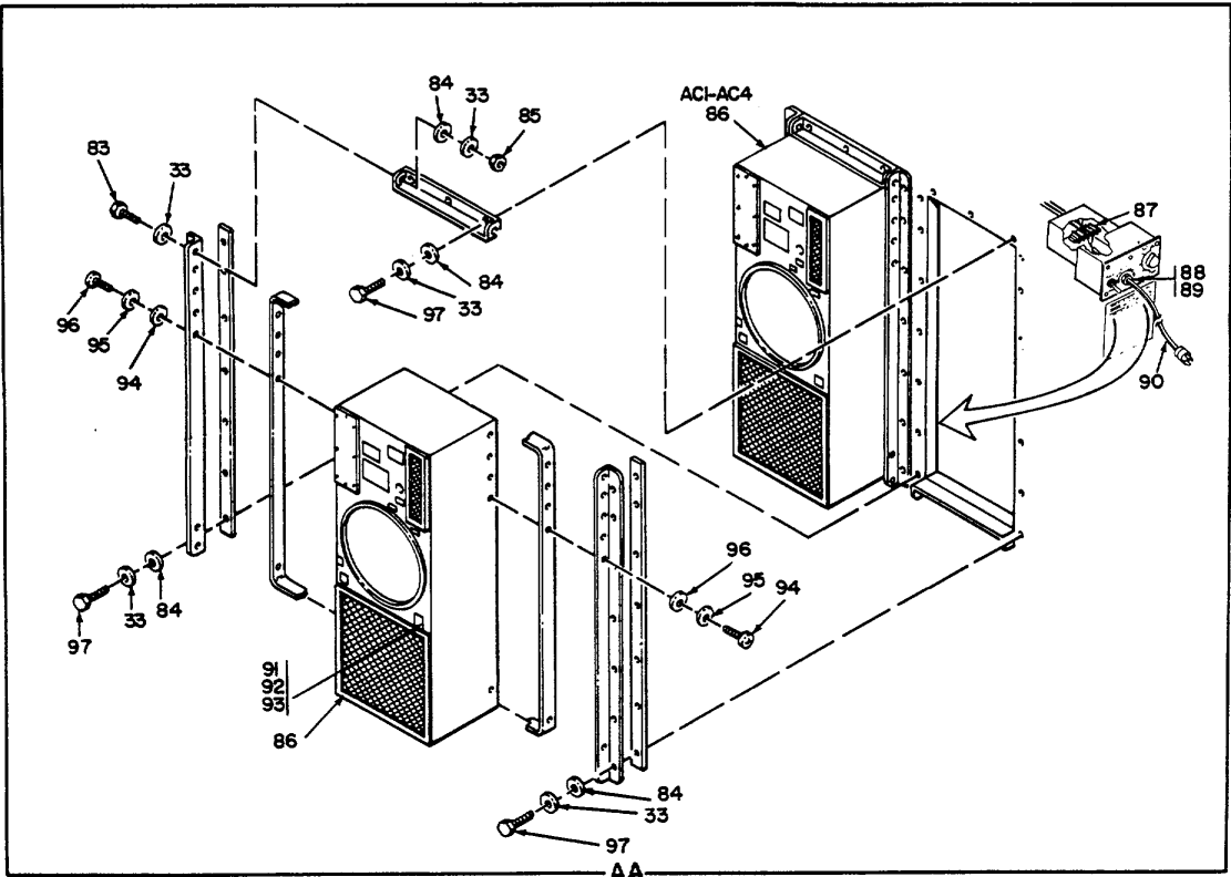
Figure 3. Electrical Installation (Sheet 7 of 7).
