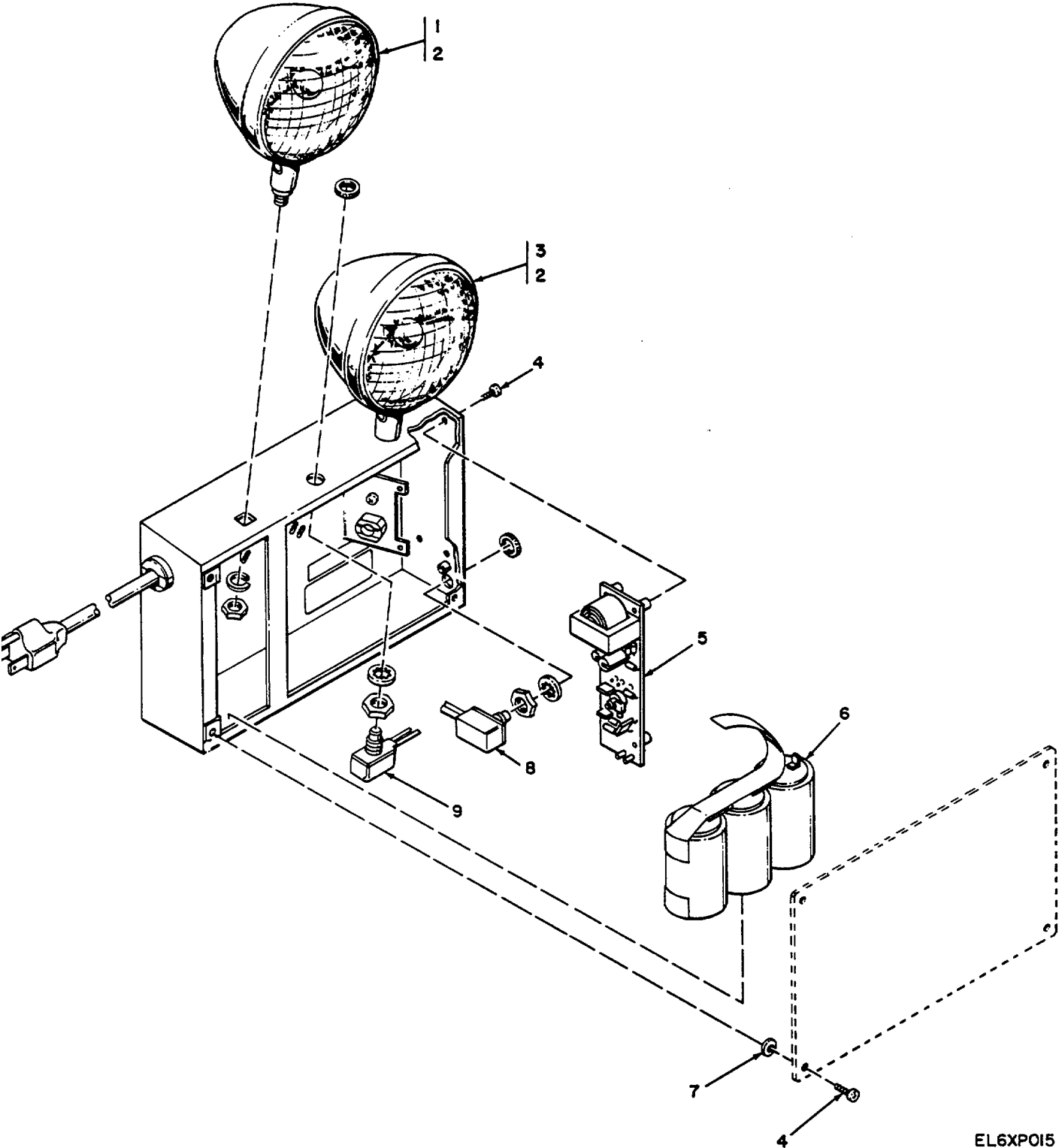
Figure 7. Emergency Lighting.
